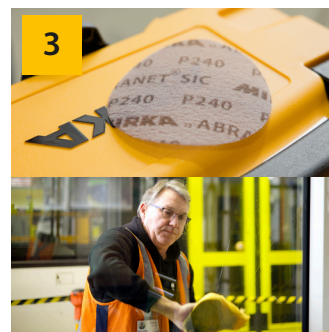
3 Sand with Deros RS 600 Sander + Abranet Sic NS 240 grit, then wipe clean
