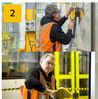
2 Sand with Deros RS 600 Sander + Abranet Sic NS 150 grit, then wipe clean
